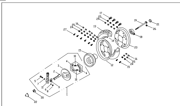
F15 FRONT WHEEL ASSY. (DRUM BRAKE)
